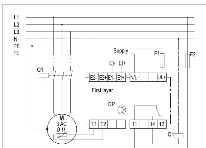
Wiring diagram
